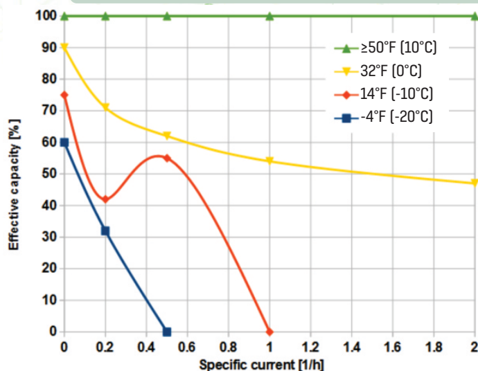
Effective capacity at various temperatures, current
